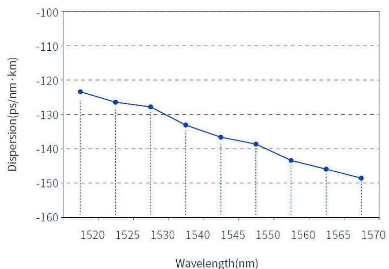
G.652 DCF Dispersion Curve
